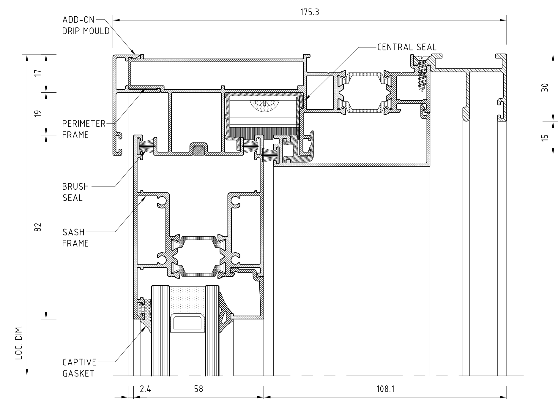
HEAD RAIL DETAIL
