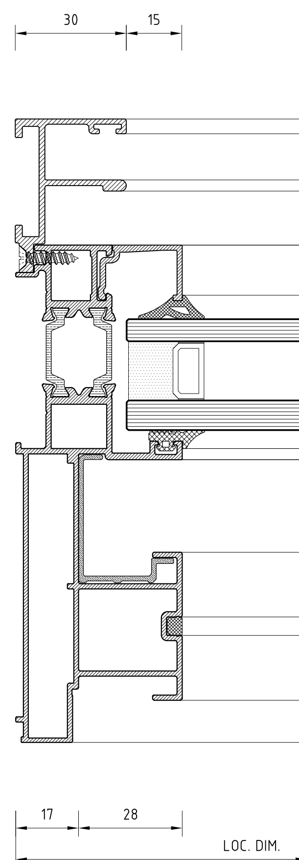
JAMB DETAIL (FIXED PANEL)
