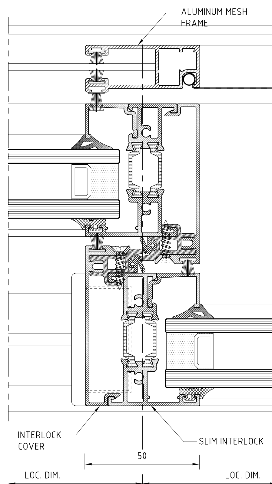
SLIM INTERLOCK DETAIL
