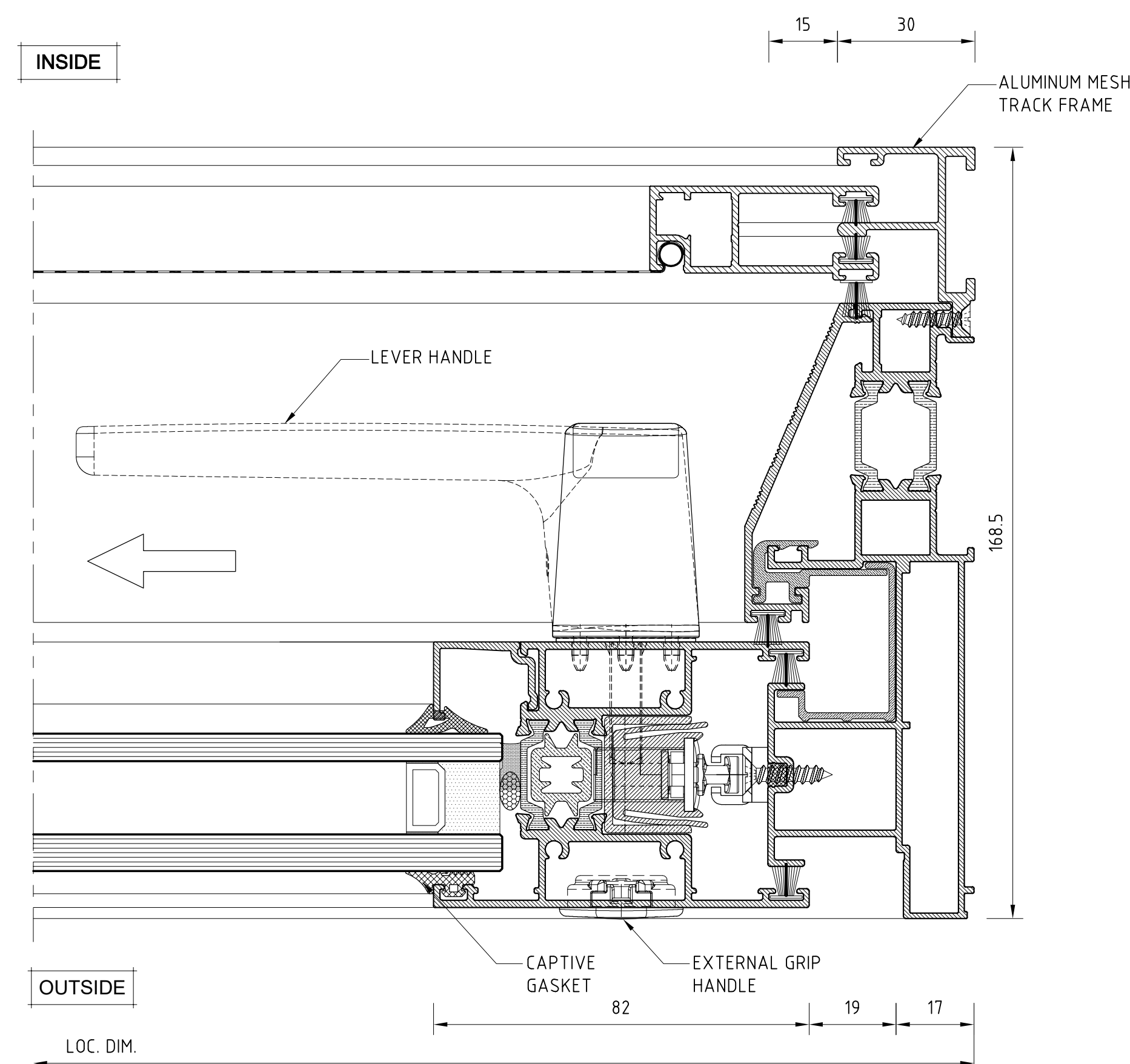
JAMB DETAIL (SLIDING PANEL)
